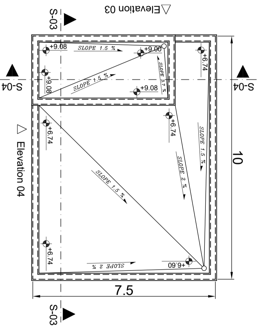
Roof PLAN
